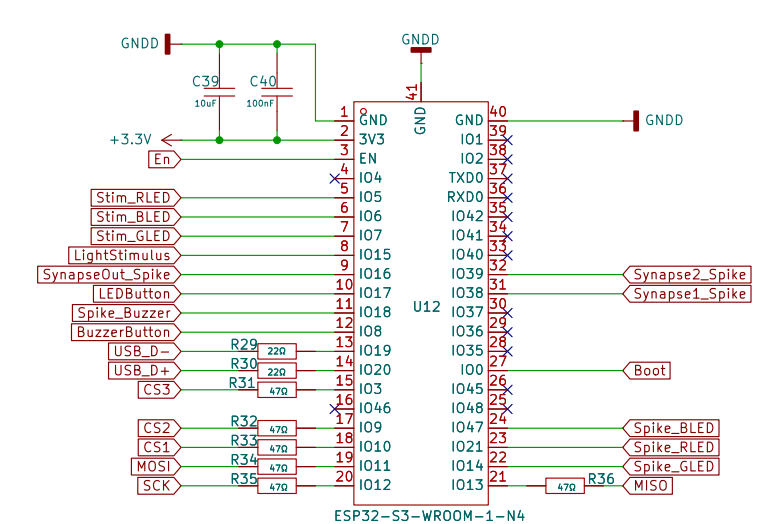
ESP32S3 WROOM1 N4
