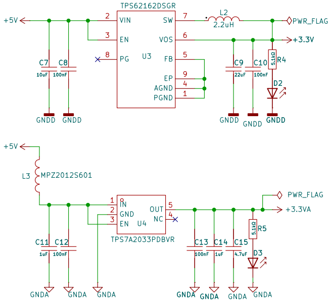
5 V to 3.3 V logic regulator
