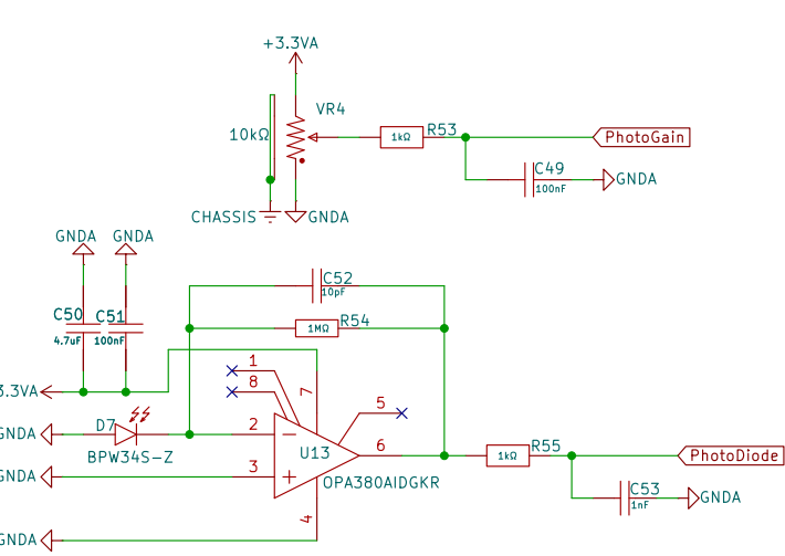
Photo-Receptor
