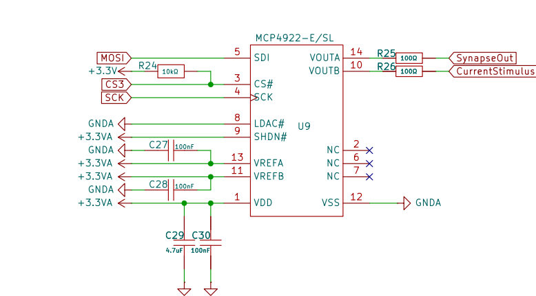
Digital to Analog Converter
