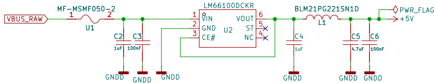
5V line
