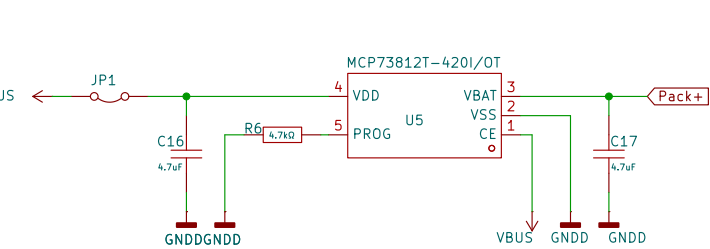
LiPo Battery Charger
