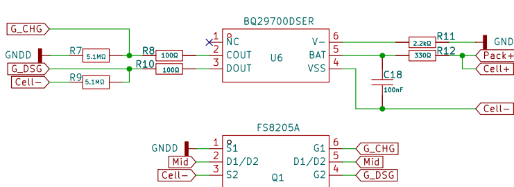
LiPo Battery Protection
