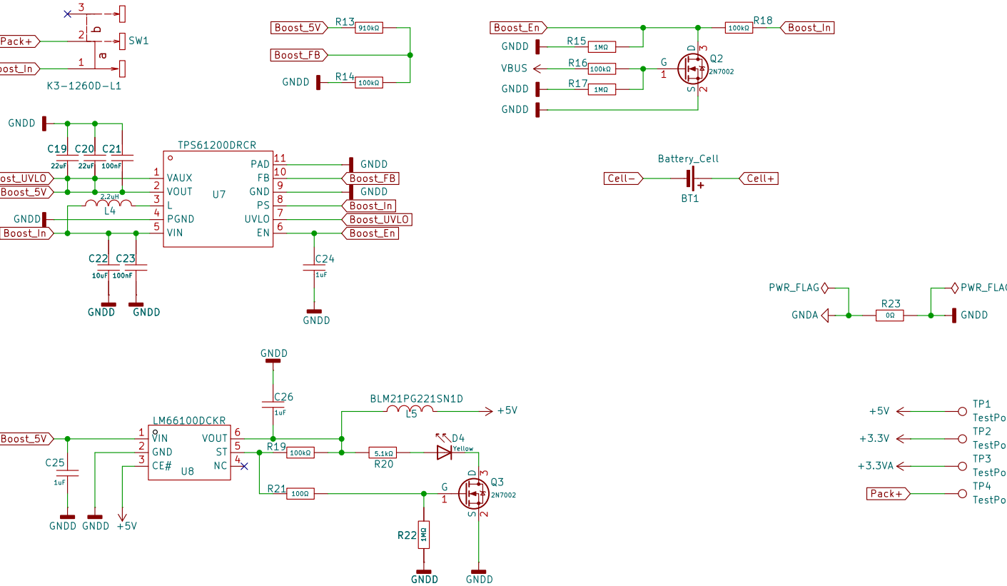
LiPo Battery Boost Converter
