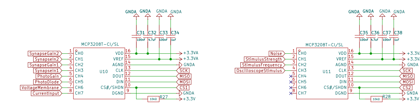
Analog to Digital Converters
